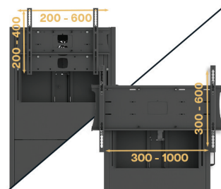
Universal screen mount is incorporated as standard - covering wide range of VESA.
