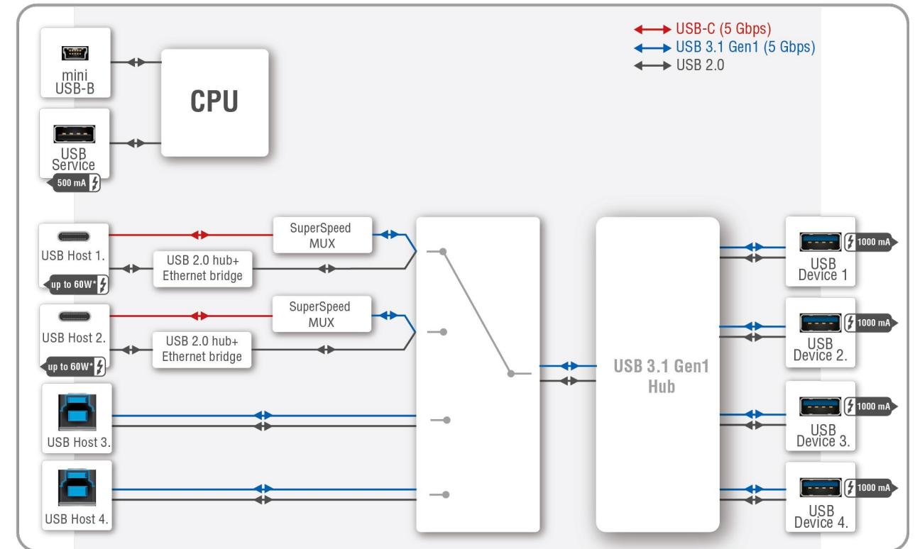
USB Port Diagram (UCX-4x2-HC30D)
