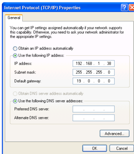
Figure 7: Internet Protocol (TCP/IP) Properties Window
