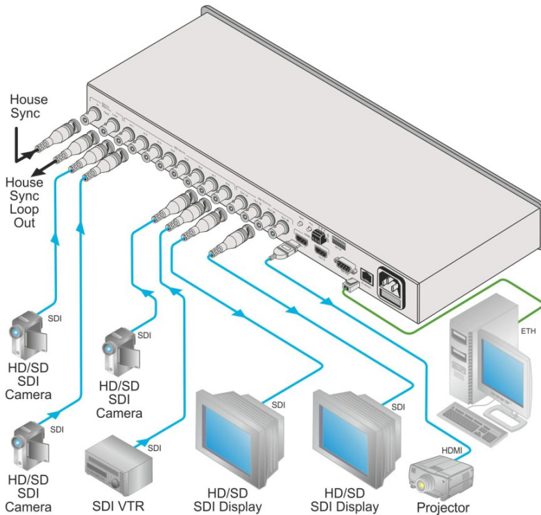
Figure 3: Connecting the VS-82HDx1 8x2 SD/HD-SDI Matrix Switcher
