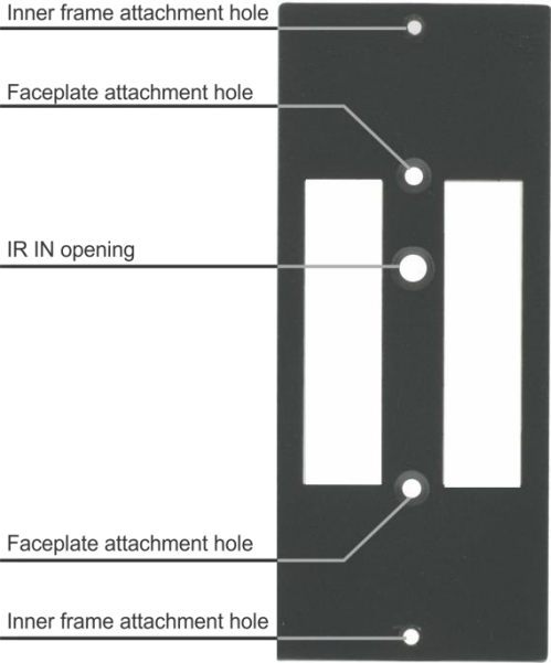
Figure 7: T-RC8IR (P/N: 80-000599)
