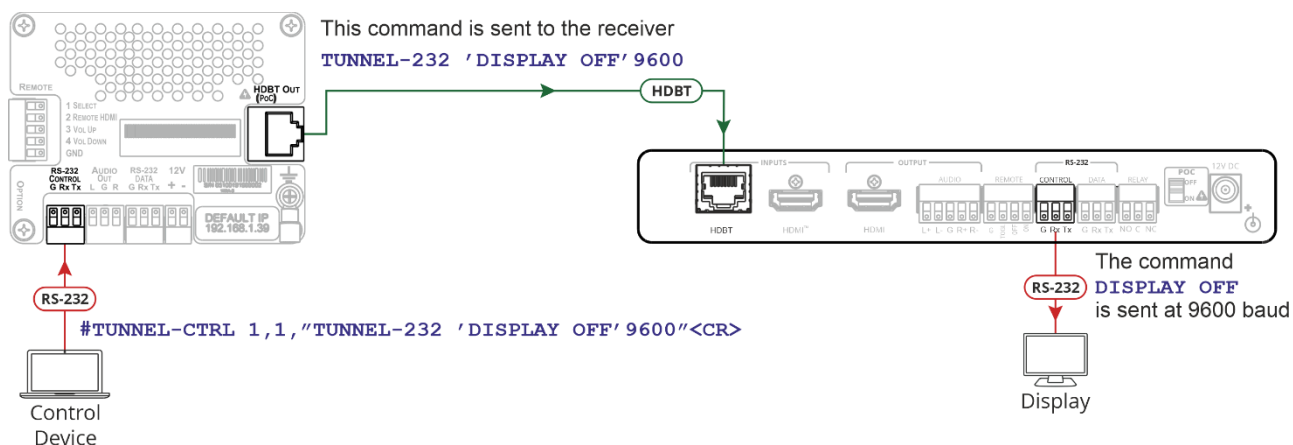
Figure 8: Controlling a Sink Device Connected to the Receiver
