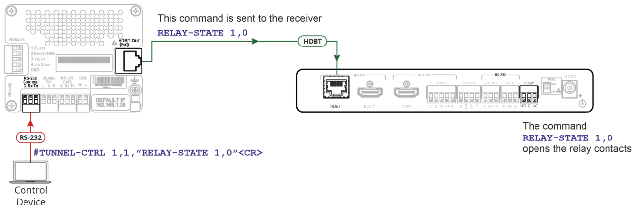
Figure 7: Controlling the Receiver via a Control System
