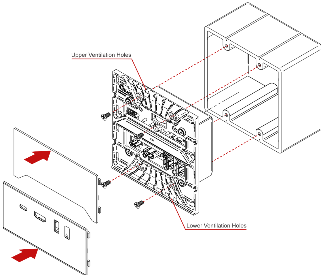
Figure 4: Mounting EXT3-C-WP-XR-T
