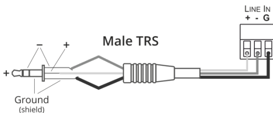
Figure 4: Connecting a Balanced 6.5mm Phone Jack
