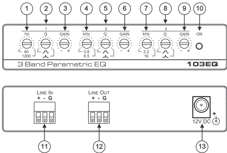
Figure 1: 103EQ 3 Band Parametric EQ
