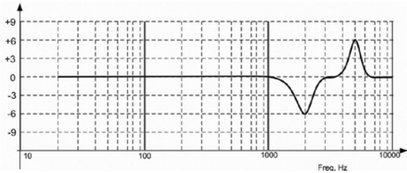
Figure 7: EQ Graph shape – Requirements
