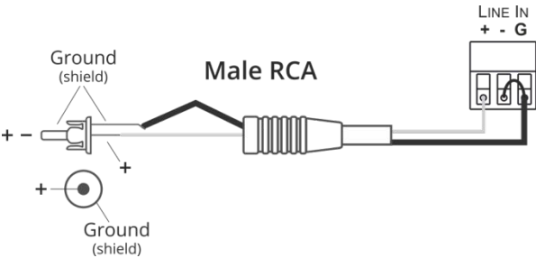
Figure 5: Connecting an Unbalanced RCA Input
