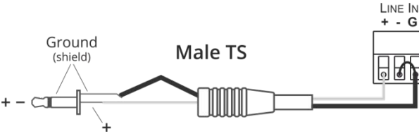
Figure 6: Connecting an Unbalanced 6.5mm Phone Jack
