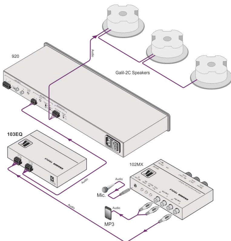
Figure 2: Connecting the 103EQ 3 Band Parametric EQ
